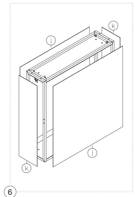
Final Assembly
